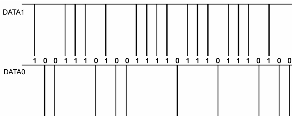
Example WIEGAND26 Output Data for the Tag Number is: 0003832762
